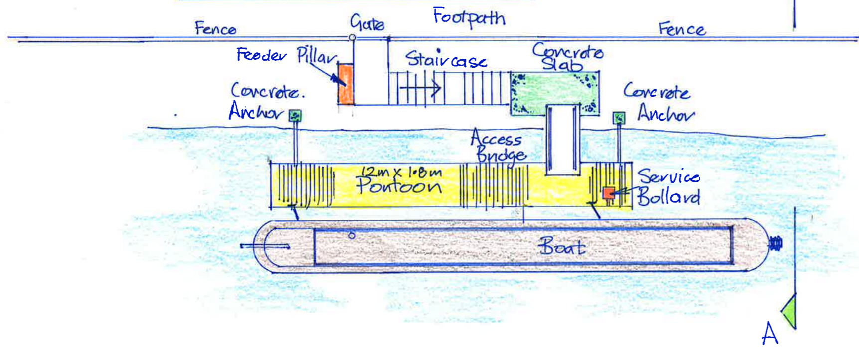
Plan of Proposed Pontoon Mooring NTS
