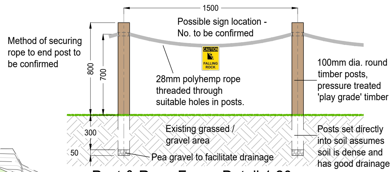
Post & Rope Fence Detail 1:20
