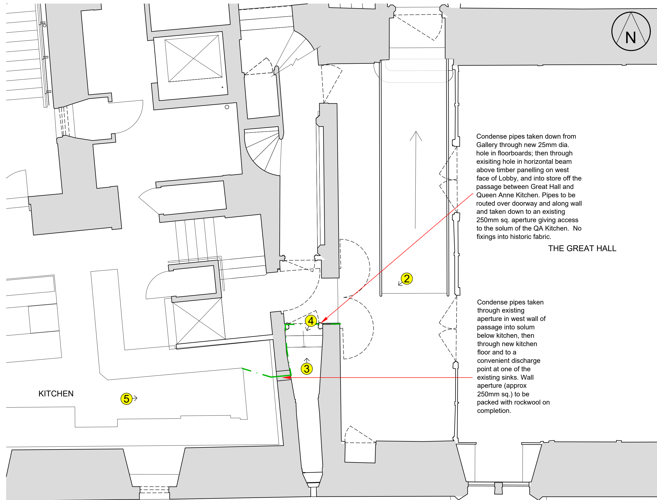
The Great Hall/Queen Anne Building - Ground Floor Plan (Scale 1:50)
