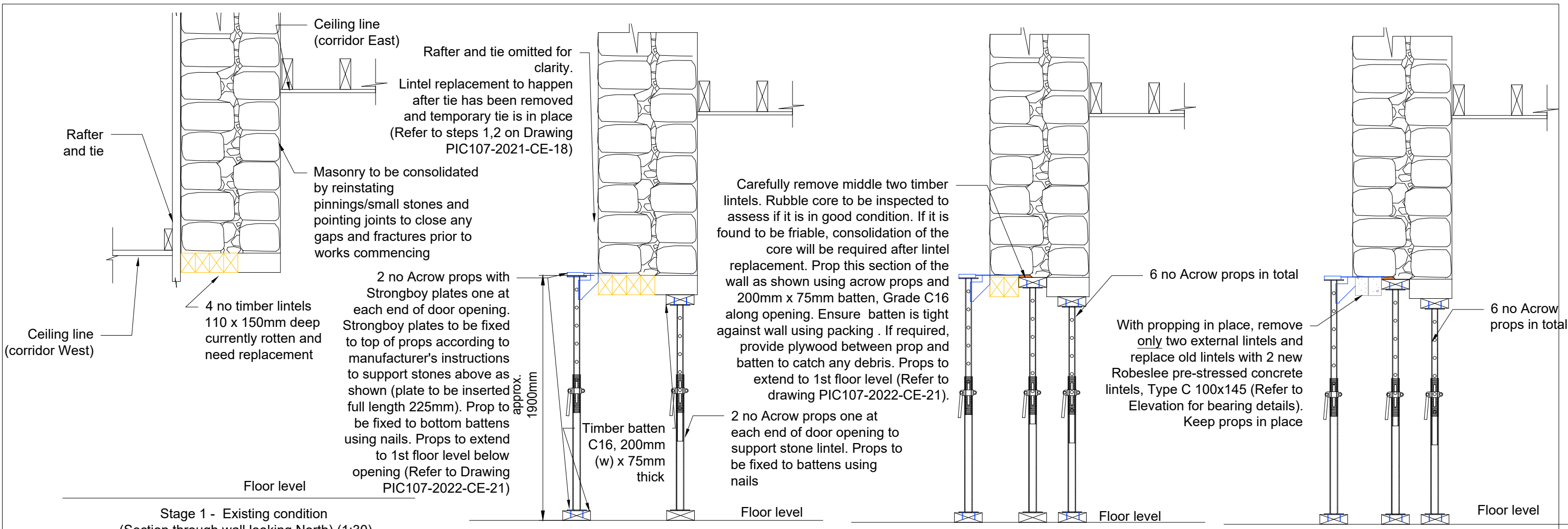
Stage 2 - Propping
