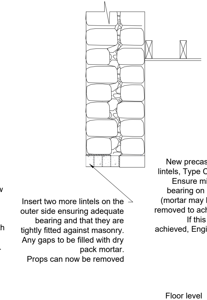
Stage 6 - Replacing outer lintels and removing propping
