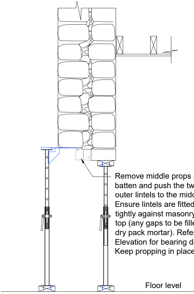
Stage 5 - Moving lintels to middle of wall
