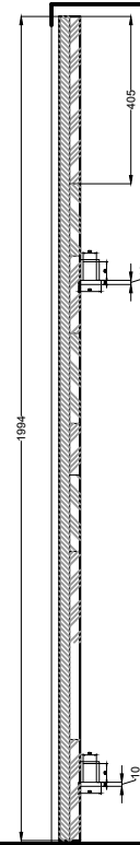
Section (1:20)
