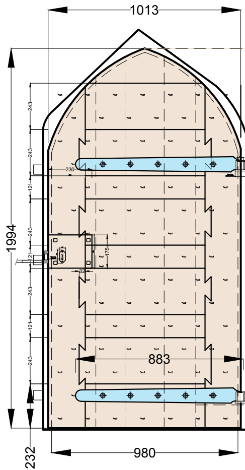
Rear Elevation (1:20)
