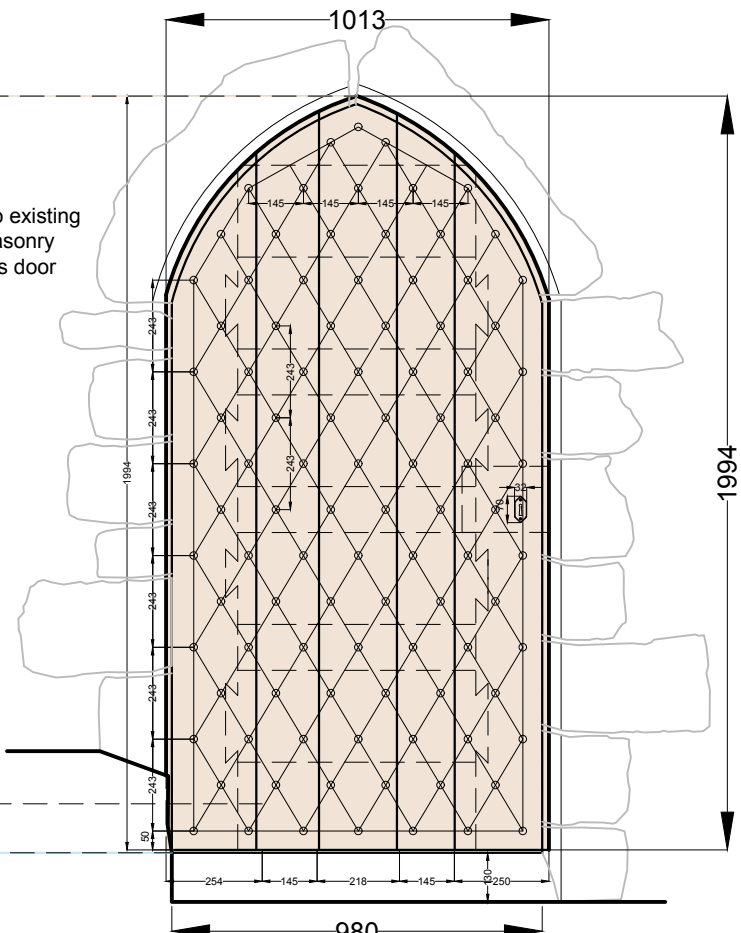
Front Elevation (1:20)
