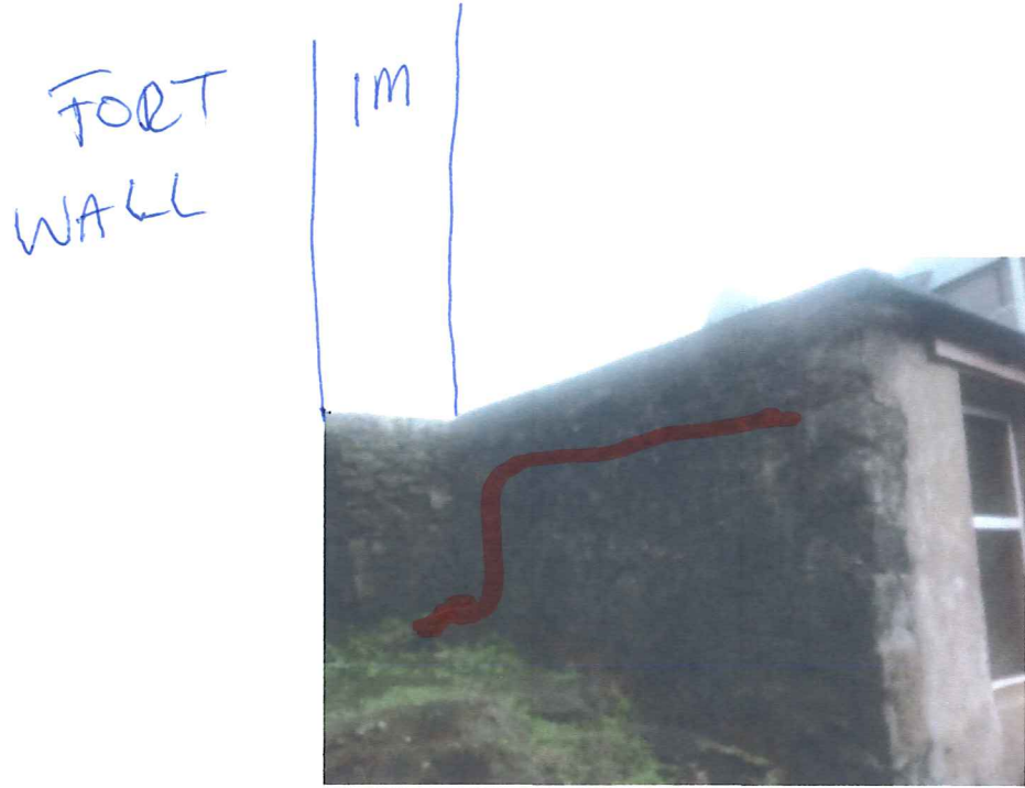
SIDE OF STORAGE BUILDING CABLE FIXED TO BUILDING
