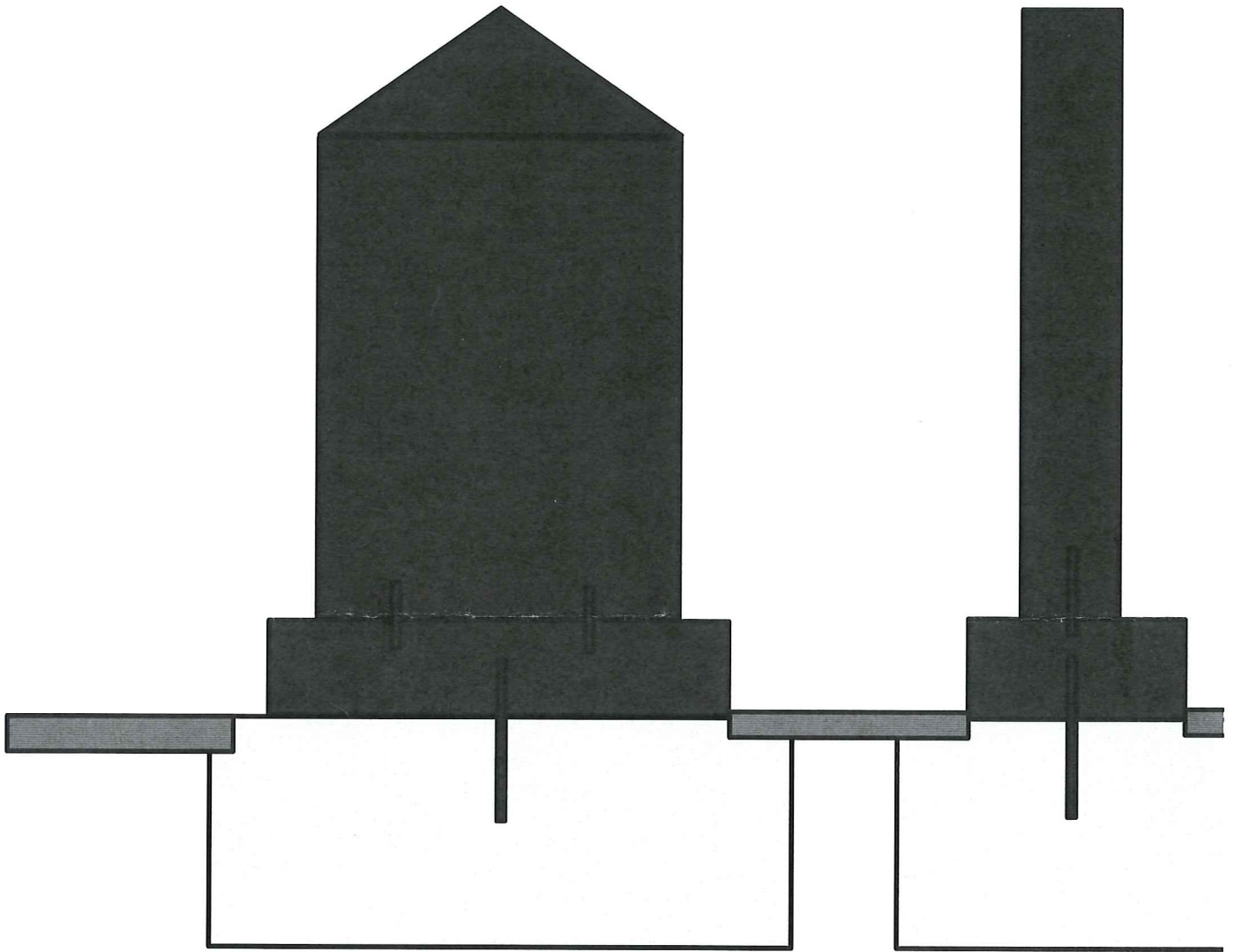
Front and side elevation of memorial of memorial showing dowels and anchor pin
