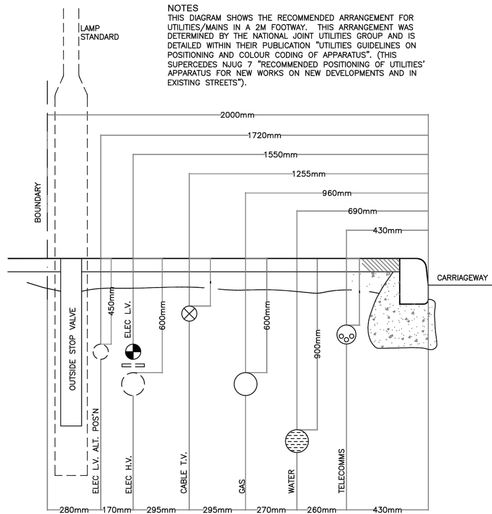
TYPICAL LOCATION OF SERVICES IN SERVICE STRIPS AND FOOTPATHS
