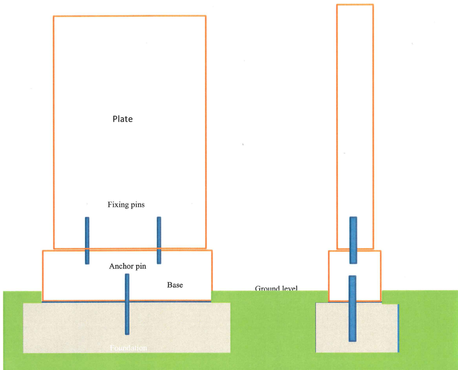
Front elevation
