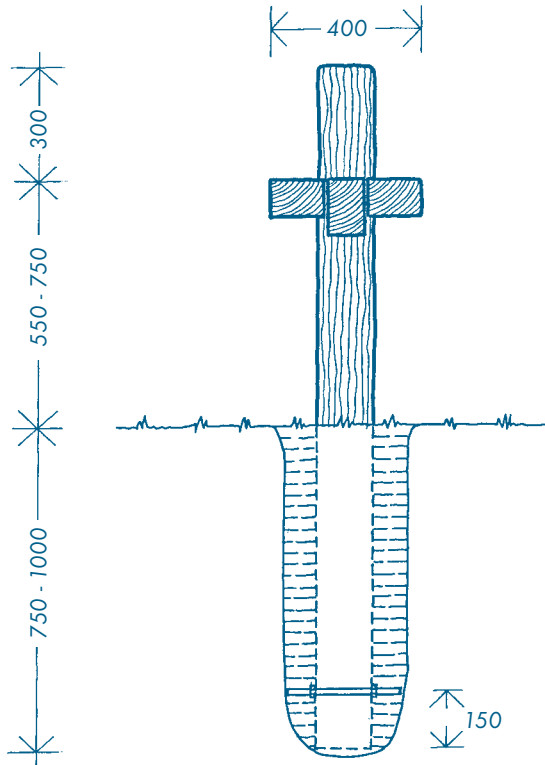
7.2C Side Elevation (Detail)
