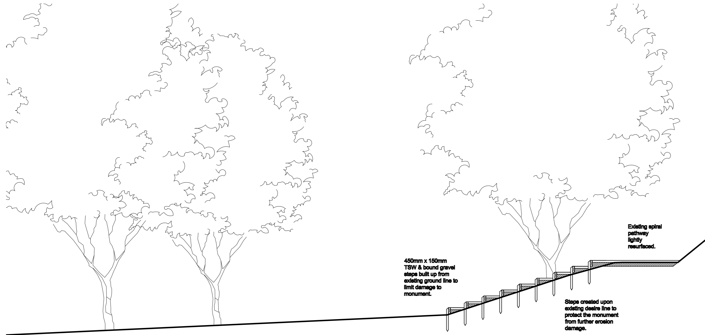
Proposed Section A - A 1:50
