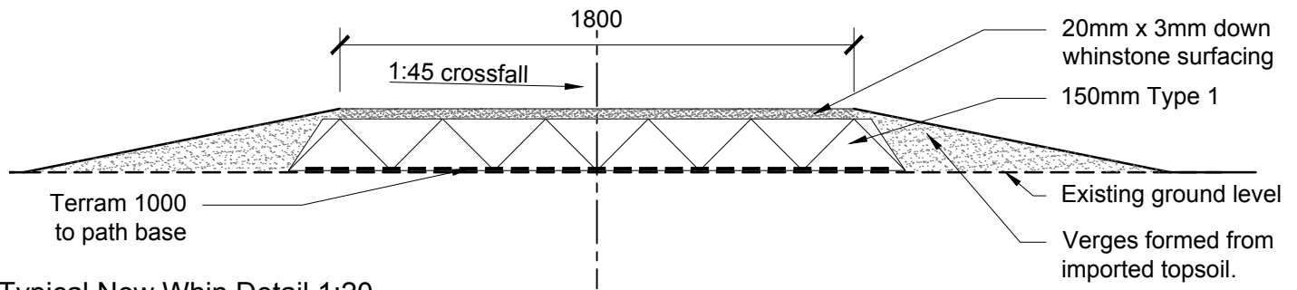
Typical New Whin Detail 1:20
