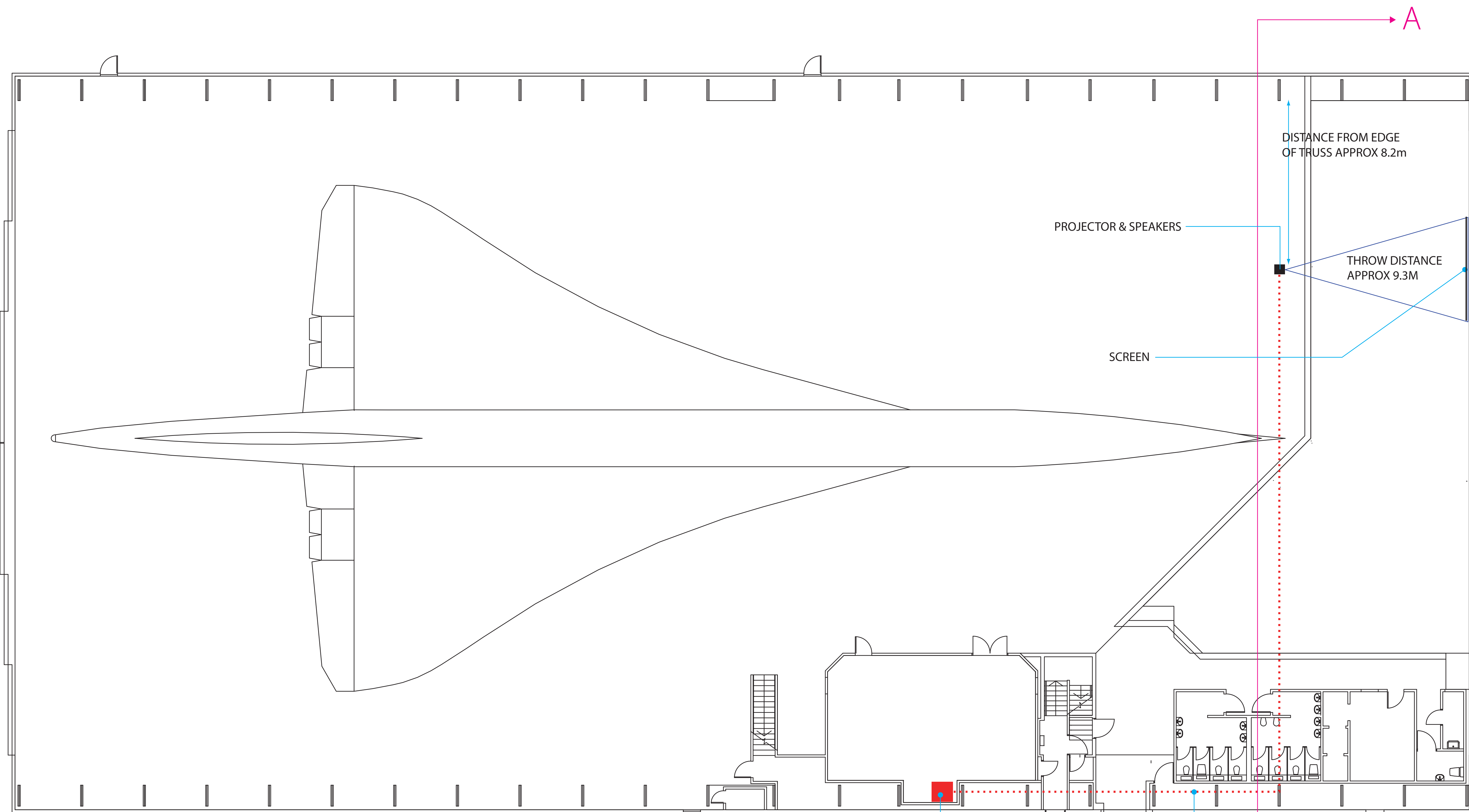
PLAN
