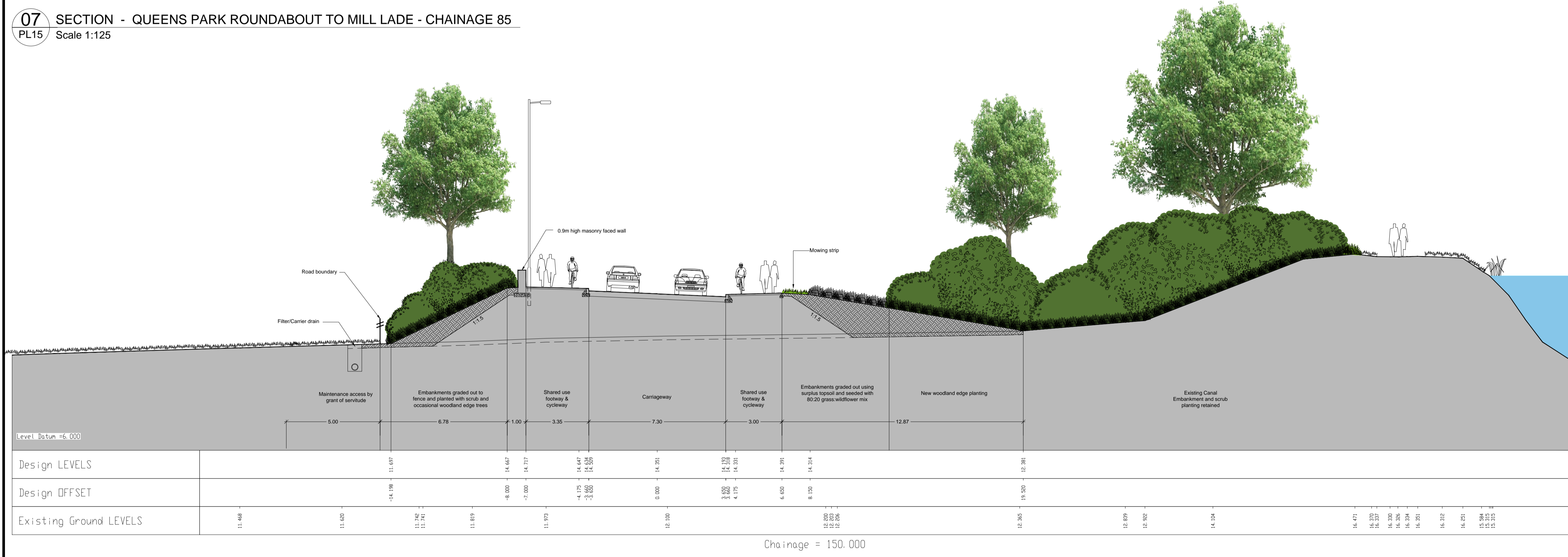
08 SECTION - QUEENS PARK ROUNDABOUT TO MILL LADE - CHAINAGE 150 PL15 Scale 1:125
