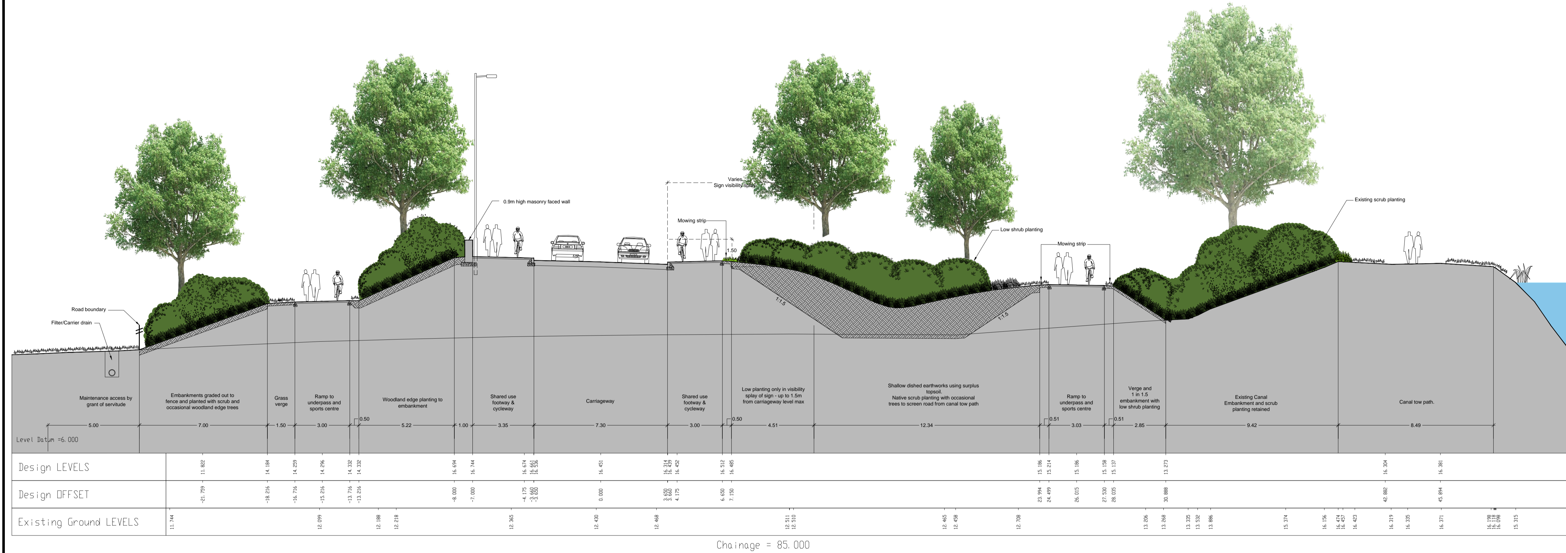
07 SECTION - QUEENS PARK ROUNDABOUT TO MILL LADE - CHAINAGE 85 PL15 Scale 1:125
