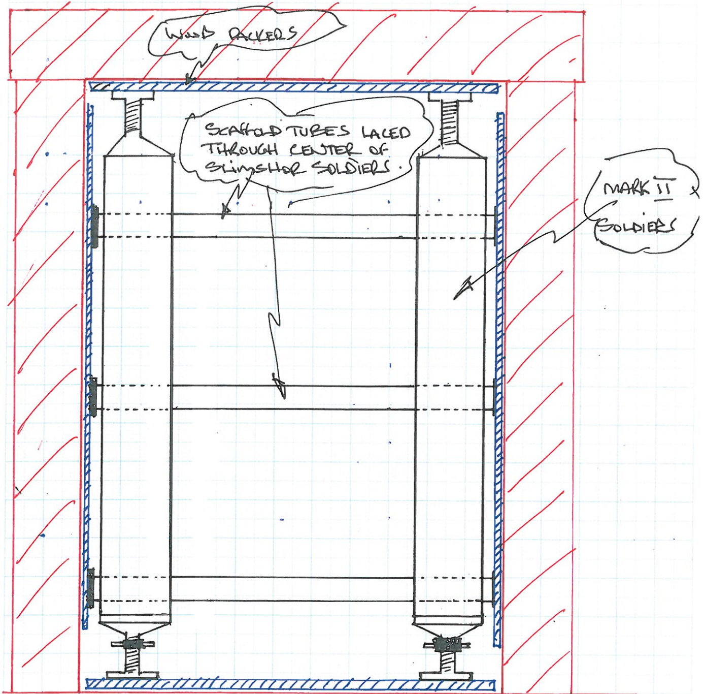
ELEVATION VIEW AT DOORWAYS 1:10
