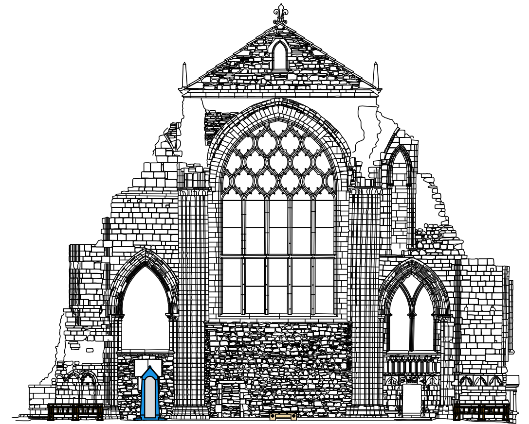
East Elevation 1:200
