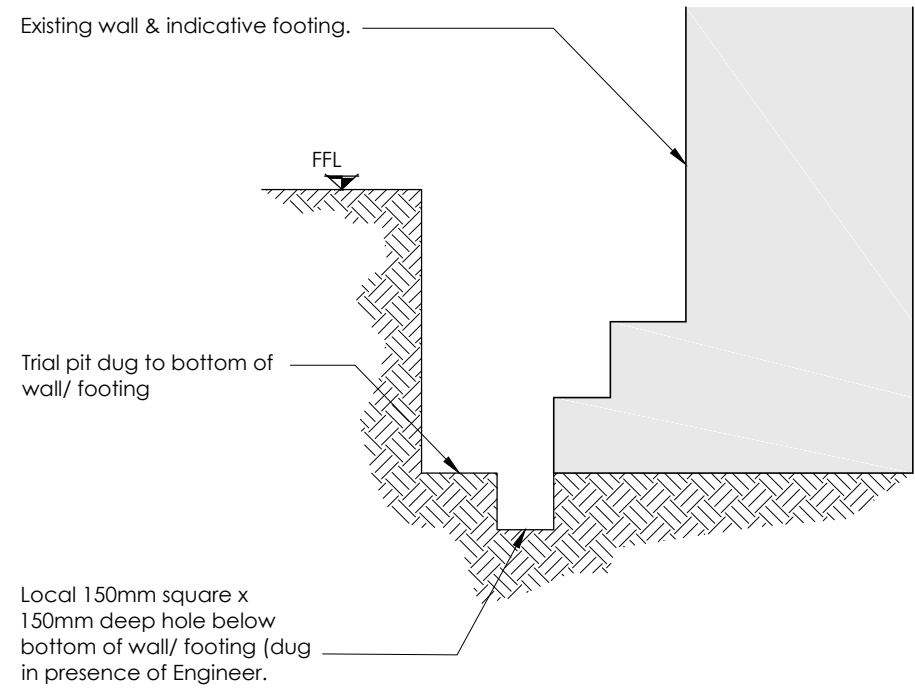
TYPICAL SECTION THROUGH TRIAL PIT 1:20
