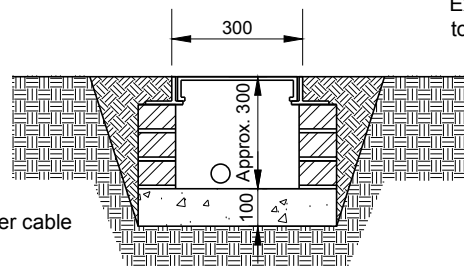
Section A-A at Proposed new manhole
