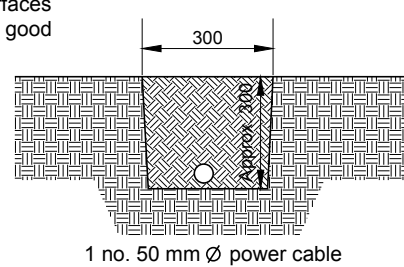
Section B-B along trench
